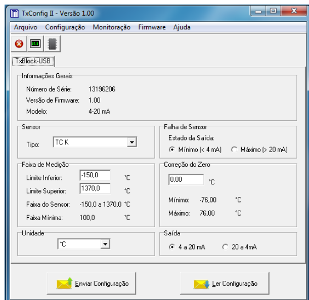
Fig. 3 – Tela principal do software TxConfig II
