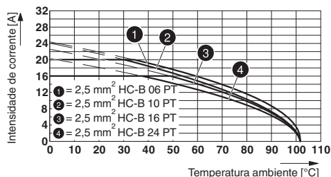
Diagrama Derating
